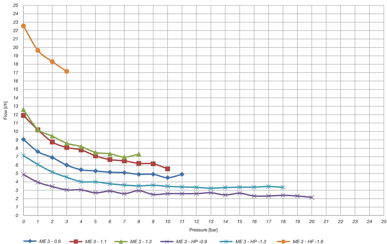
Performance curve
