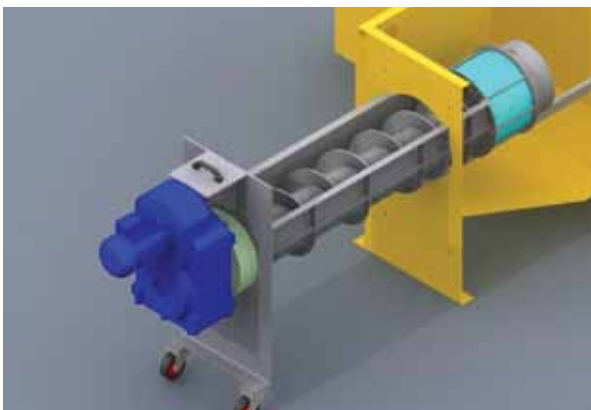
User-friendly compactor screw and washing head. Head can be removed to provide safe and easy access to the cleaning brushes without the need for a crane (optional design arrangement).
